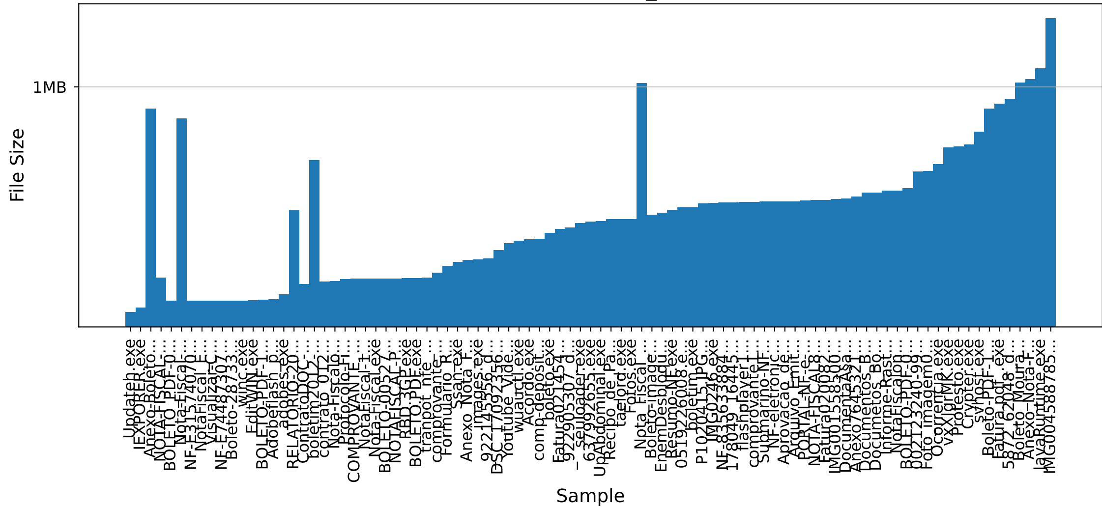
Size distribution of Cluster2_Size100 dataset
